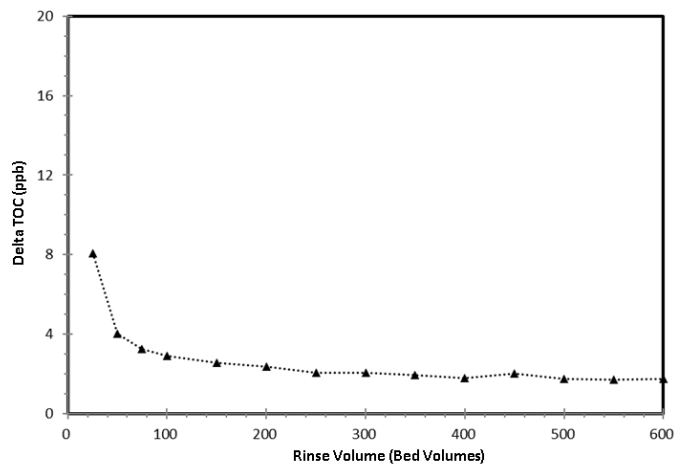
Figure 2: TOC Rinse-down
