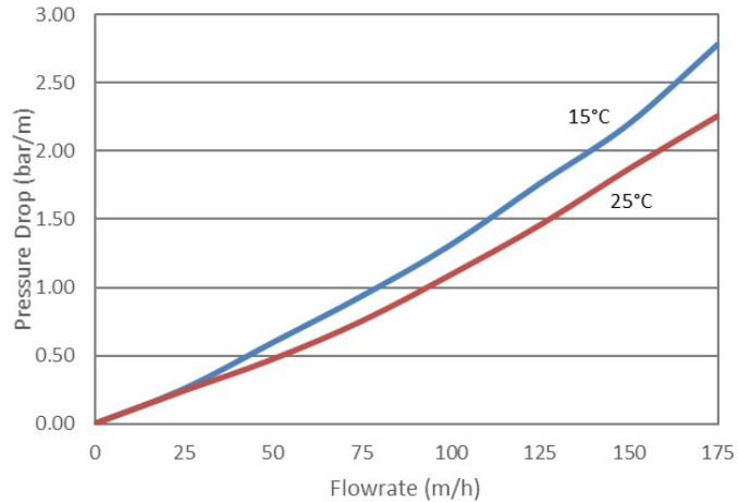
Figure 1: Pressure Drop
