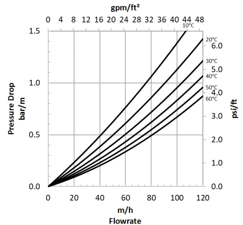
Figure 2: Pressure Drop
