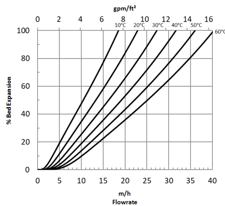
Figure 1: Backwash Expansion
