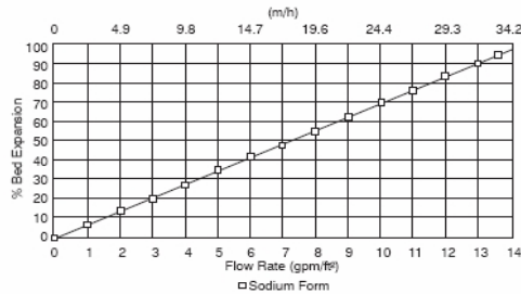
Figure 1: Backwash Expansion
