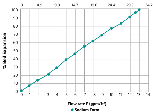
Figure 1. Backwash Expansion
