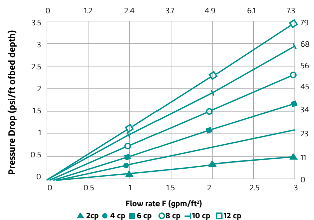
Figure 2. Pressure Drop
