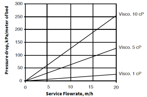
Figure 2: Pressure Drop
