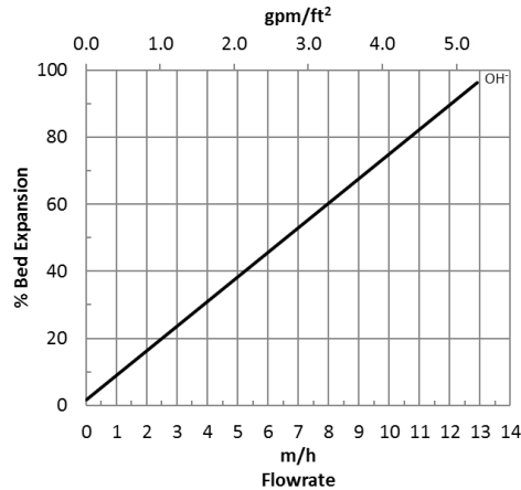
Figure 1: Backwash Expansion
