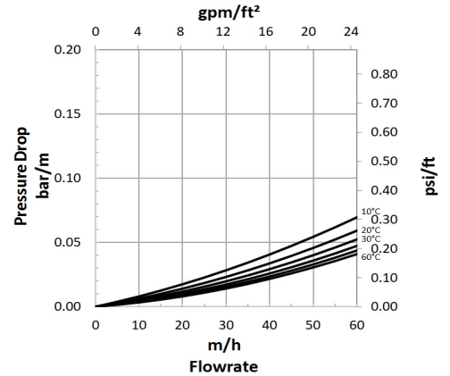
Figure 1b: Pressure Drop
