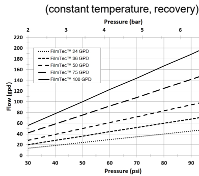
Figure 1: Impact of Pressure on Target Permeate Flow (constant temperature, recovery)
